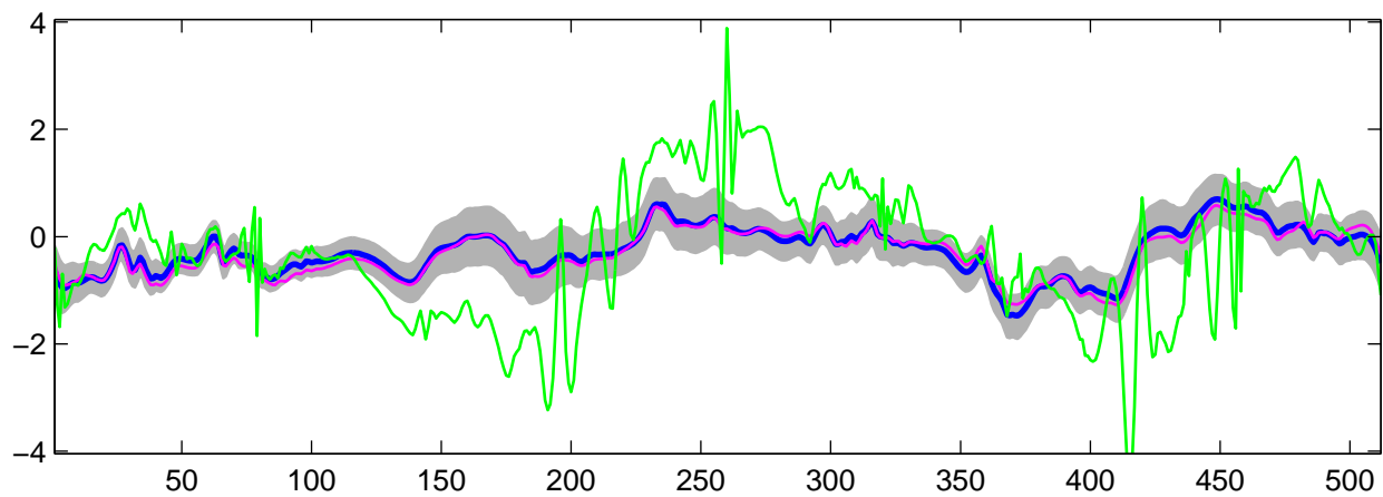
Estimated C_2(t) using R-WFMM: t_1 data, run 6
