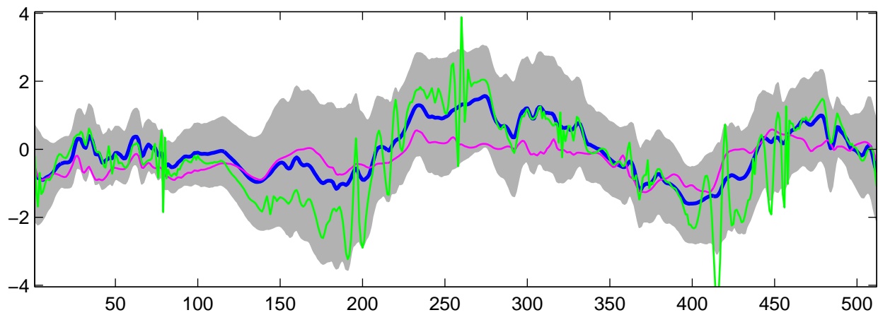
Estimated C_2(t) using G-WFMM: t_1 data, run 6
