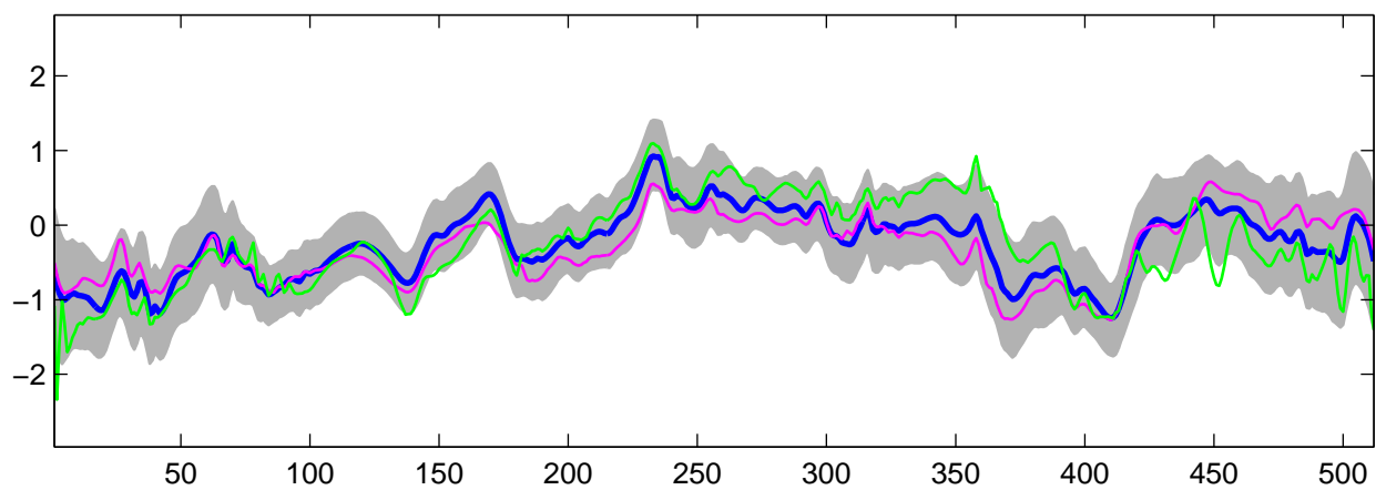
Estimated C_2(t) using R-WFMM: t_2 data, run 6
