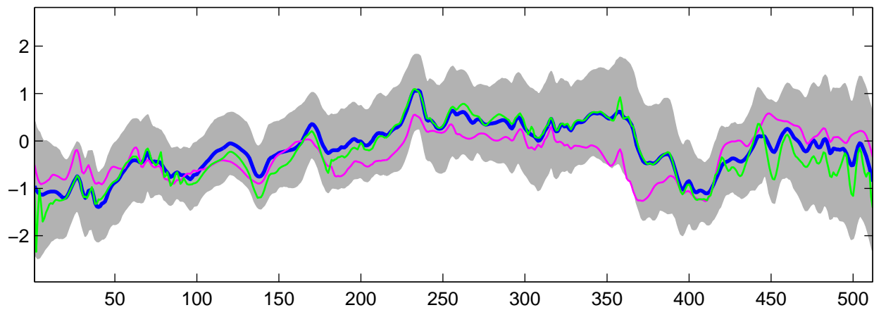
Estimated C_2(t) using G-WFMM: t_2 data, run 6
