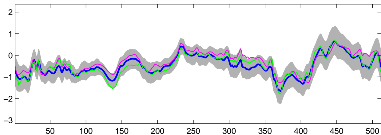
Estimated C_2(t) using R-WFMM: t_3 data, run 6
