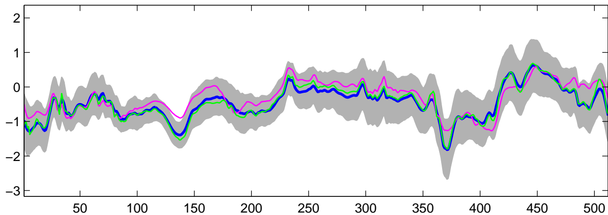
Estimated C_2(t) using G-WFMM: t_3 data, run 6
