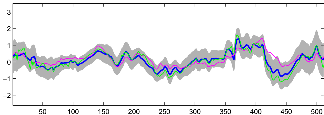
Estimated C_3(t) using R-WFMM: DE data, run 6
