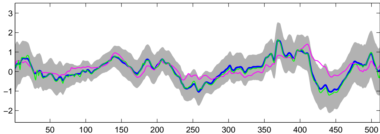
Estimated C_3(t) using G-WFMM: DE data, run 6
