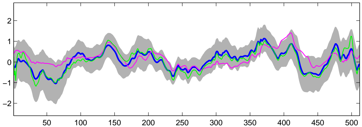
Estimated C_3(t) using R-WFMM: Normal data, run 6
