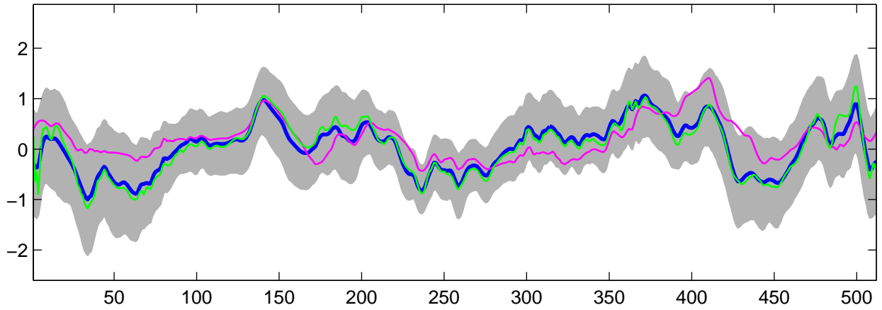
Estimated C_3(t) using G-WFMM: Normal data, run 6
