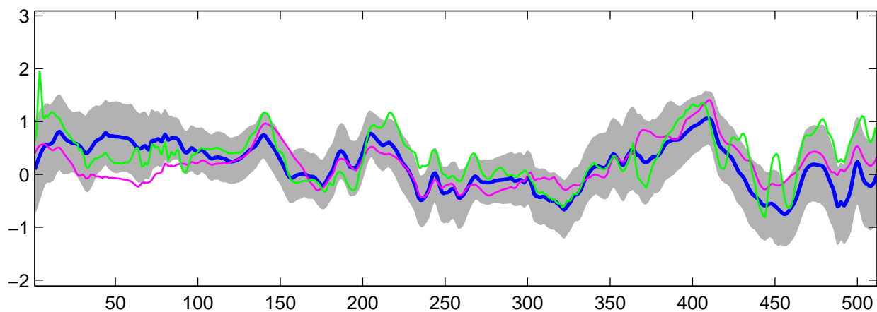
Estimated C_3(t) using R-WFMM: t_2 data, run 6
