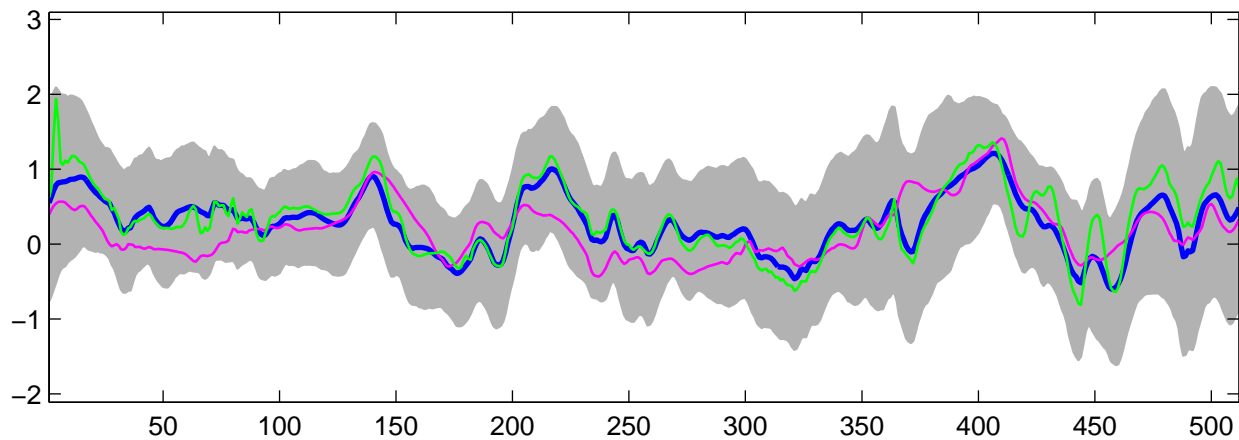
Estimated C_3(t) using G-WFMM: t_2 data, run 6
