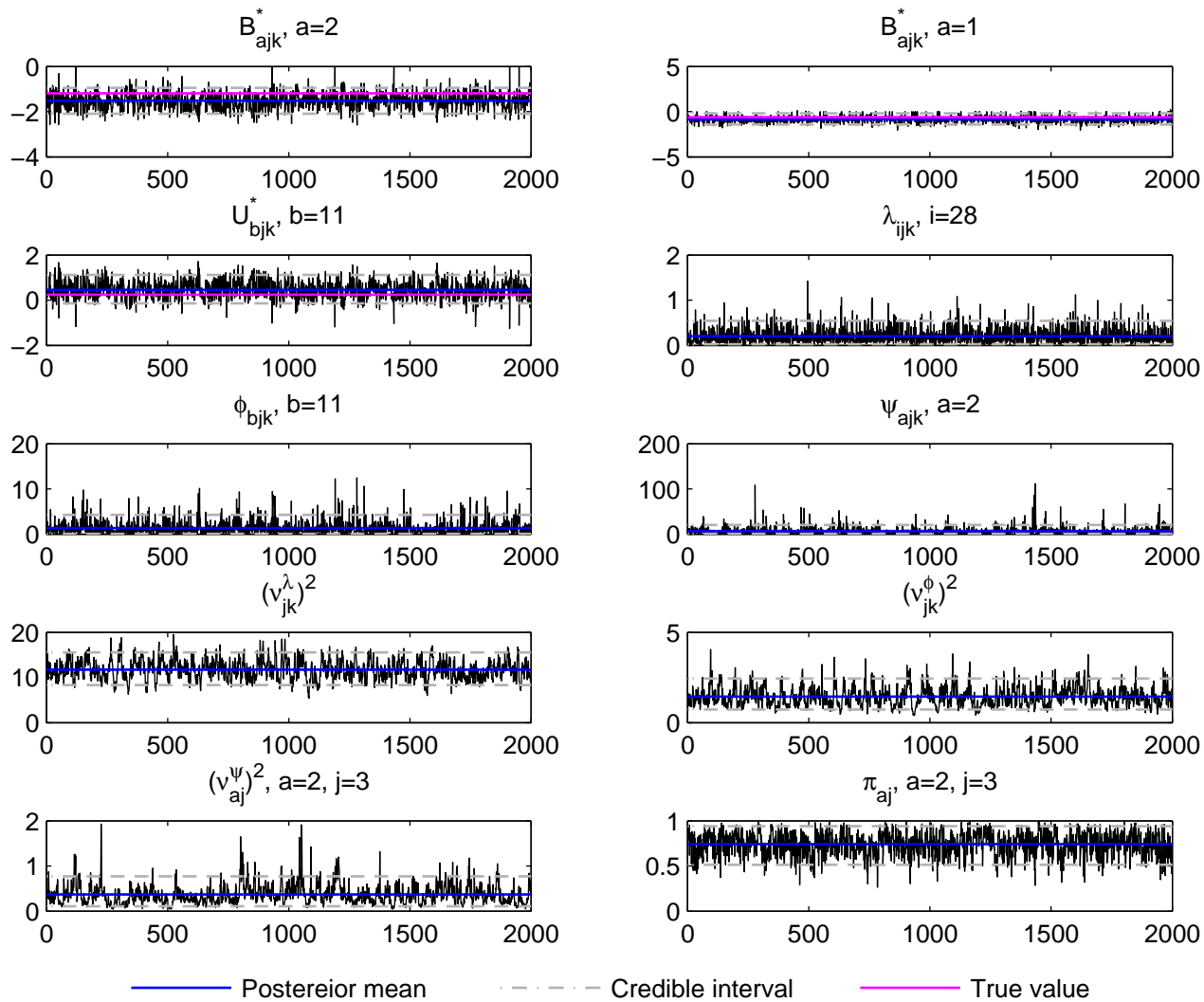
Trace plot, j=3, k=2 , DE data, simulation run 6
