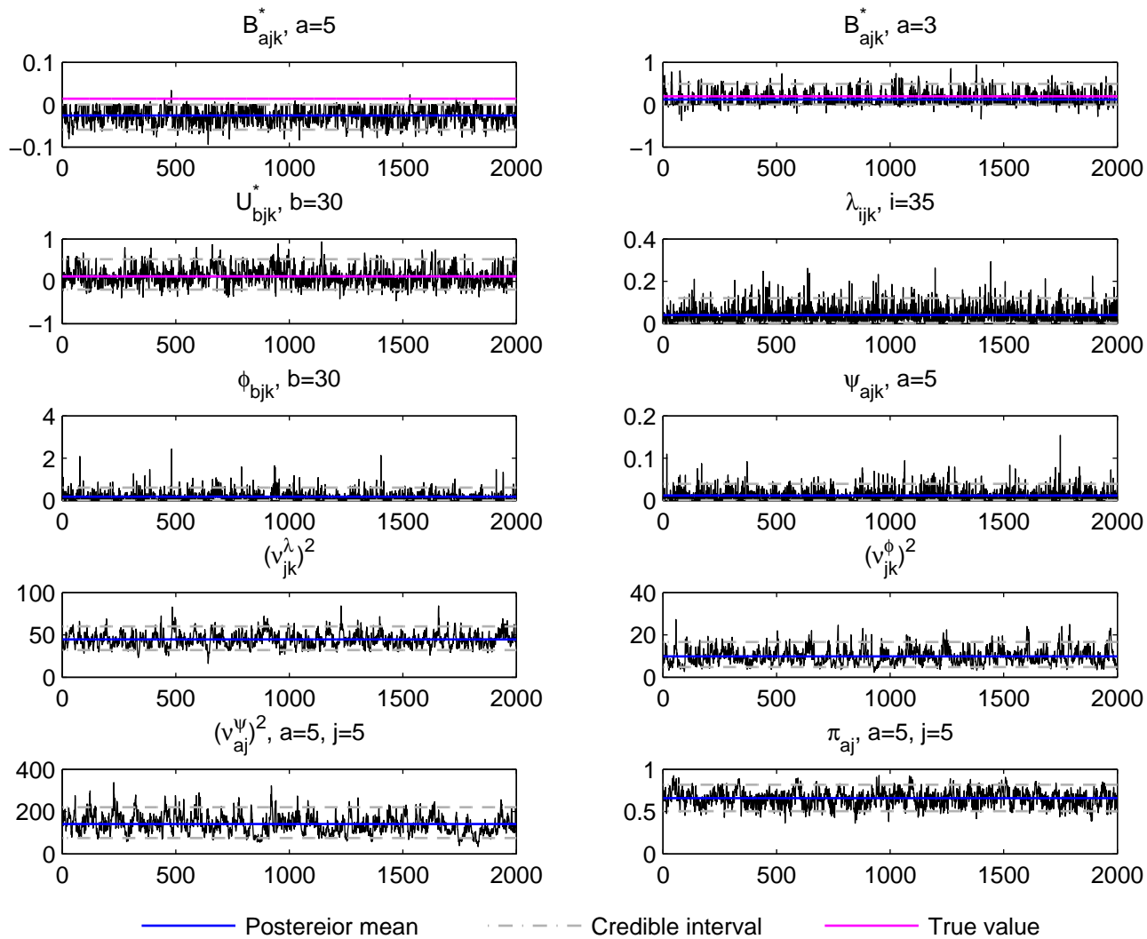
Trace plot, j=5, k=2 , Normal data, simulation run 6
