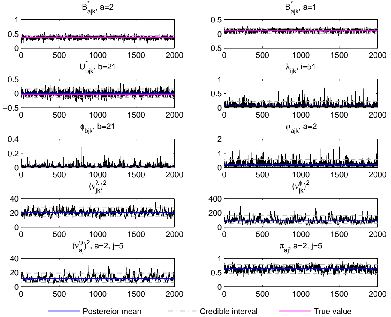
Trace plot, j=5, k=2, t_j data, simulation run 6
