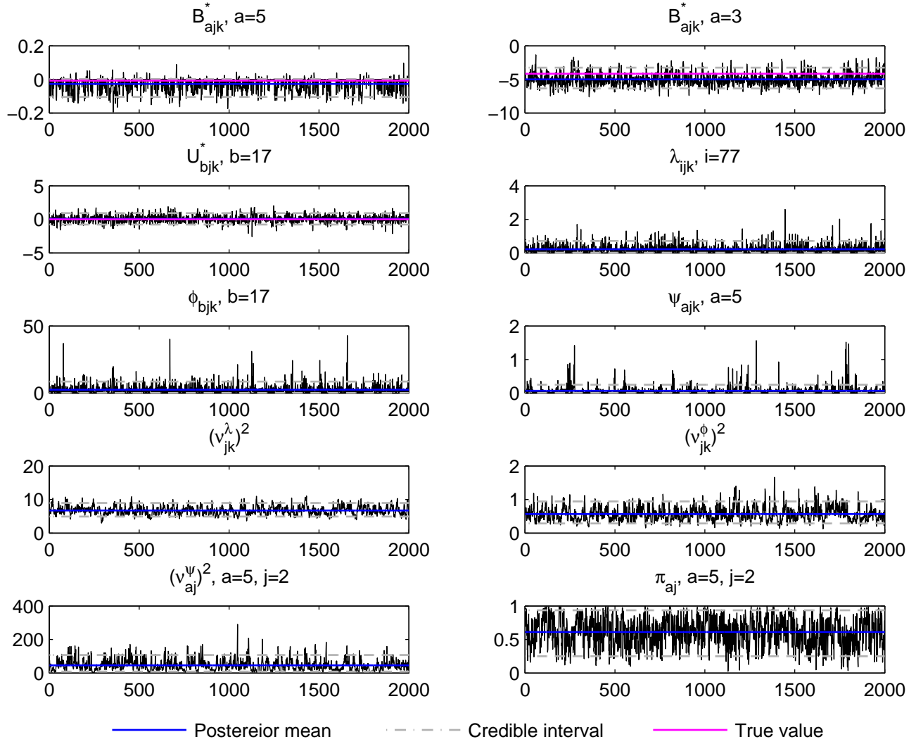
Trace plot, j=2, k=4, t_3 data, simulation run 6
