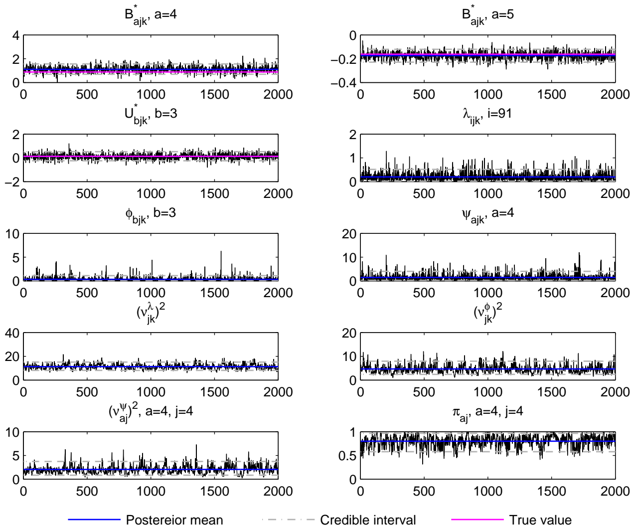
Trace plot, j=4, k=3 , DE data, simulation run 6
