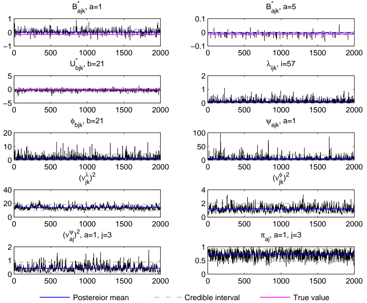
Trace plot, j=3, k=6, t_i data, simulation run 6
