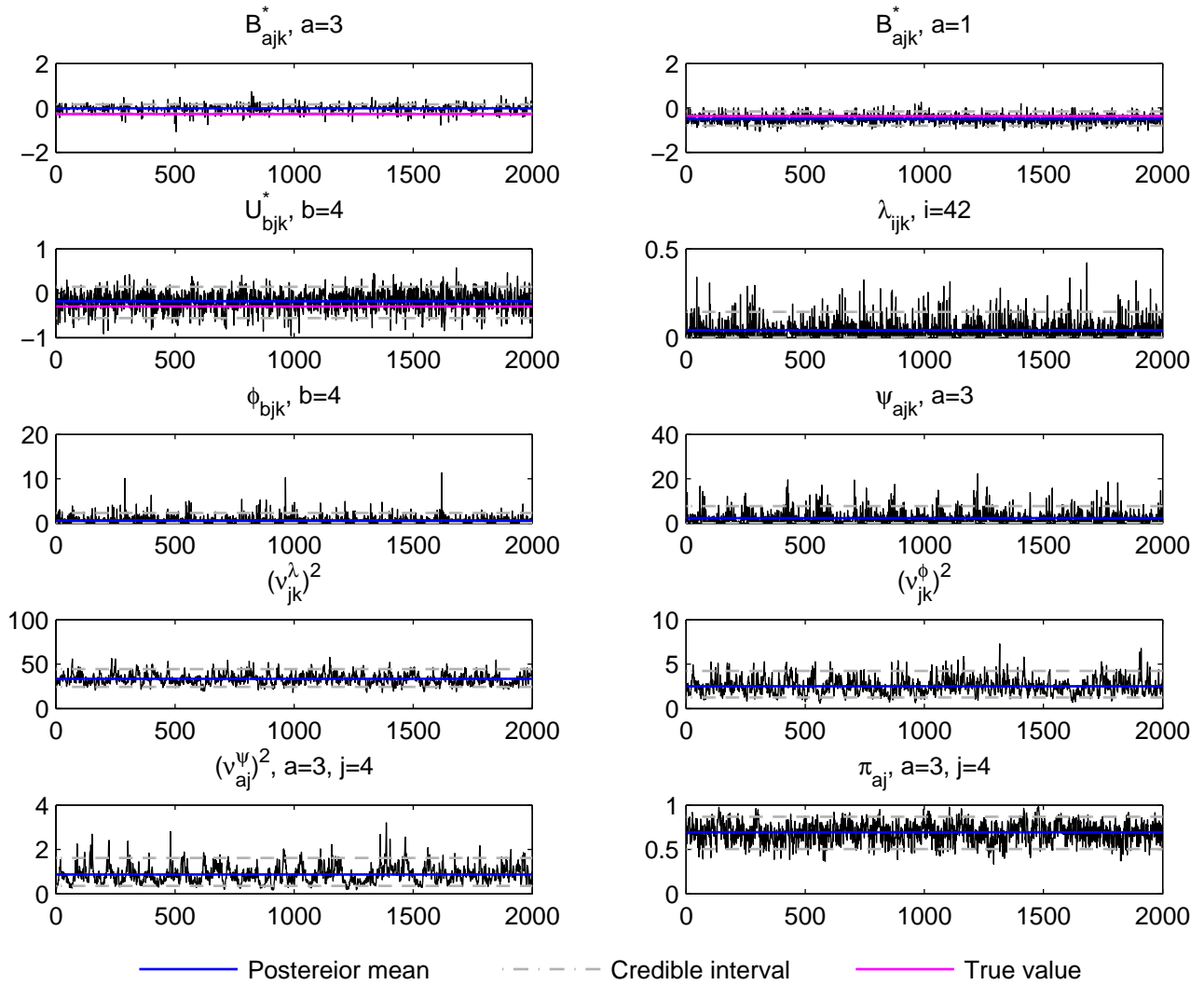
Trace plot, j=4, k=2, t_2 data, simulation run 6
