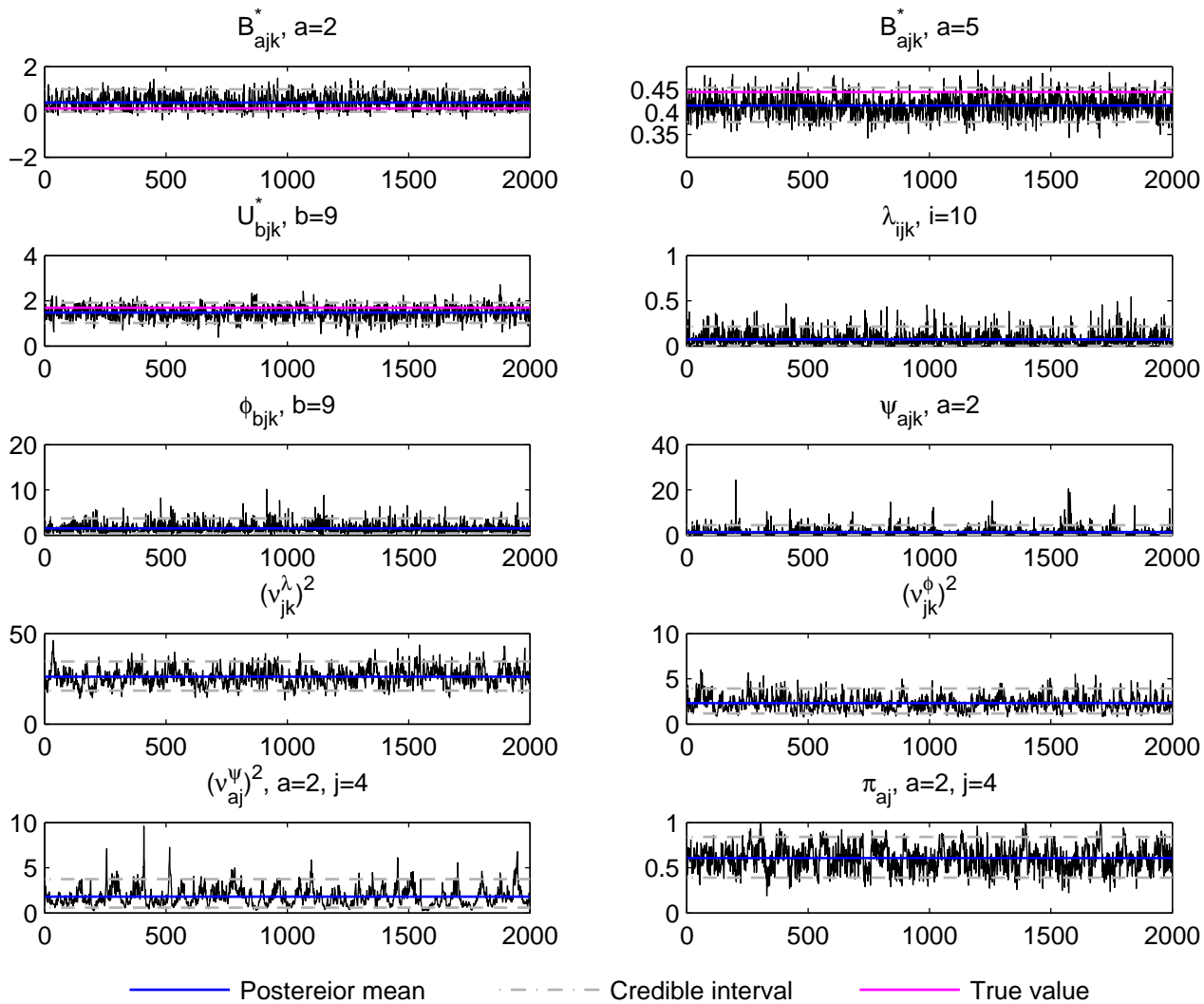
Trace plot, j=4, k=2 , DE data, simulation run 6
