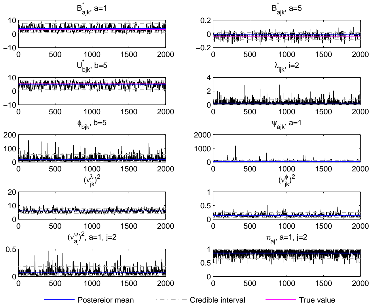
Trace plot, j=2, k=1 , Normal data, simulation run 6
