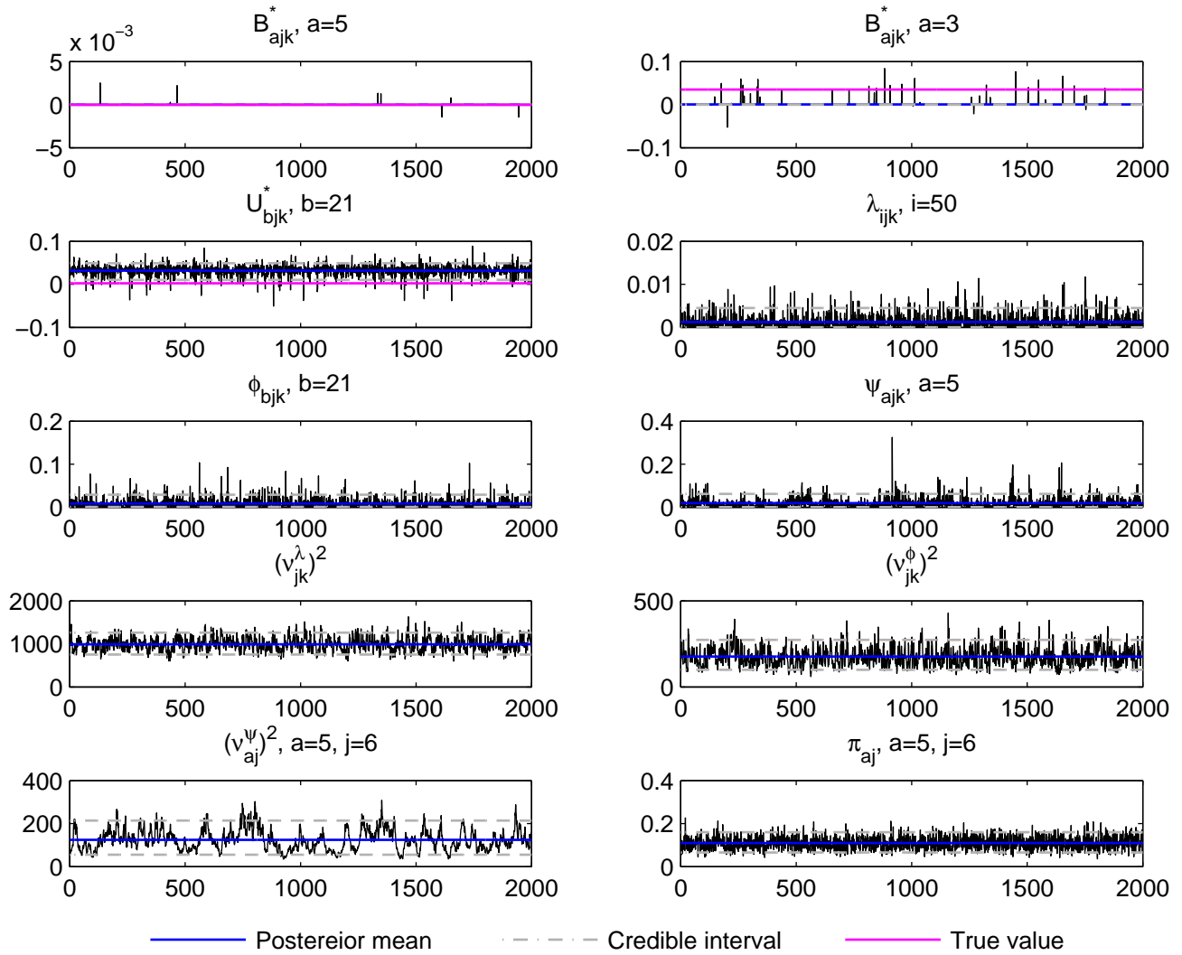
Trace plot, j=6, k=2, t_i data, simulation run 6
