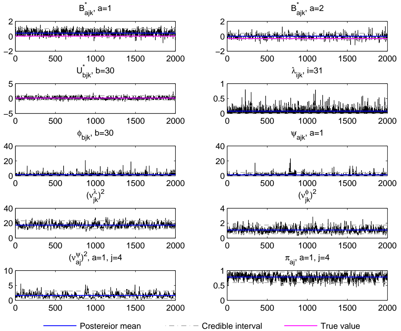
Trace plot, j=4, k=1, t_3 data, simulation run 6
