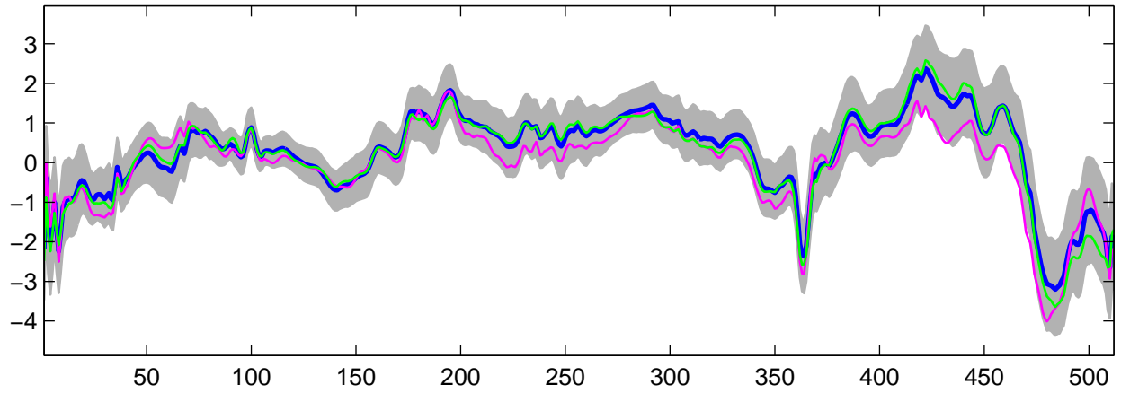
Estimated U_{10}(t) using G-WFMM: DE data, run 6
