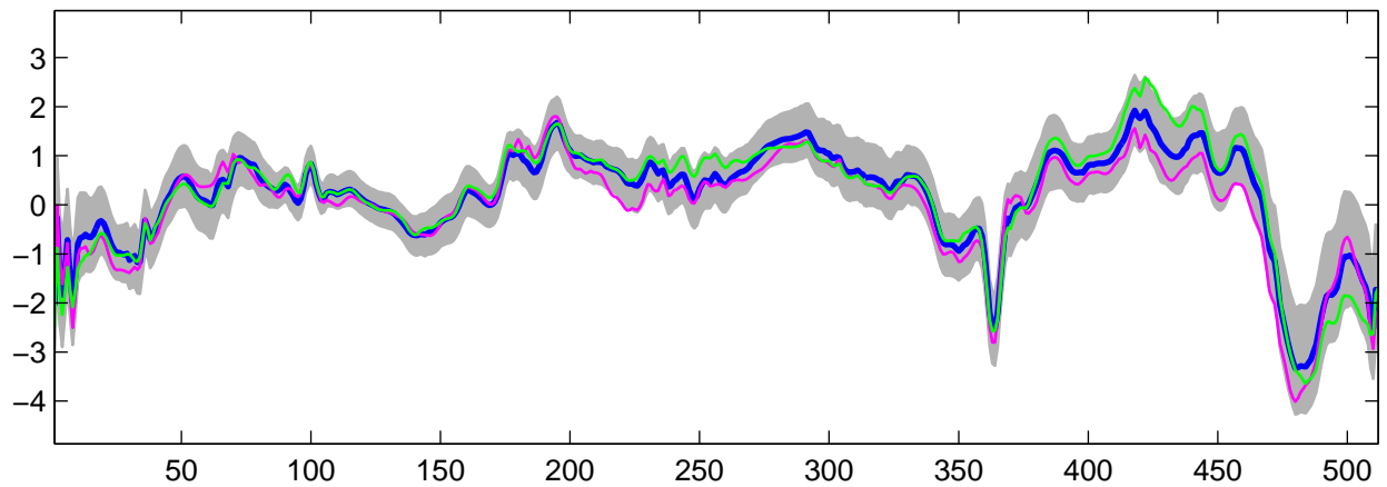
Estimated U_{10}(t) using R-WFMM: DE data, run 6
