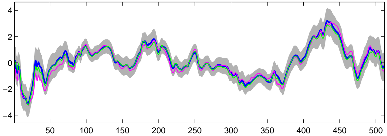
Estimated U_{10}(t) using G-WFMM: Normal data, run 6
