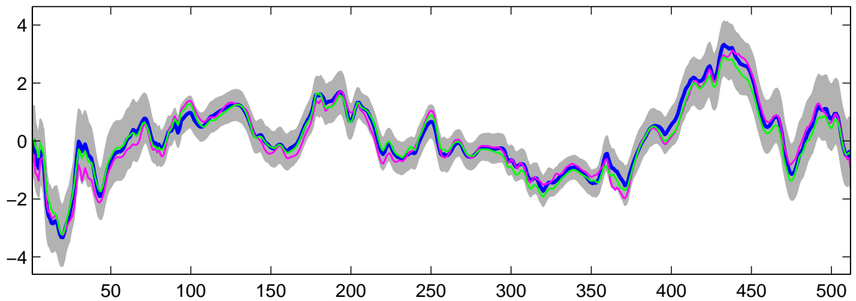
Estimated U_{10}(t) using R-WFMM: Normal data, run 6
