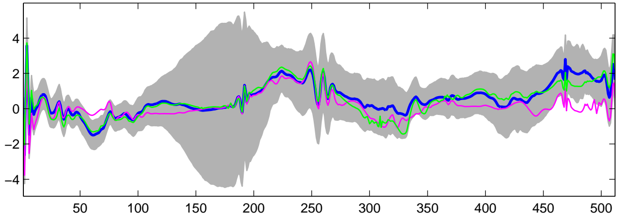
Estimated U_{10}(t) using G-WFMM: t_1 data, run 6
