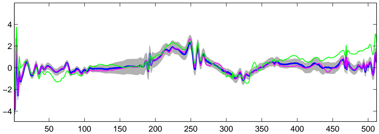
Estimated U_{10}(t) using R-WFMM: t_1 data, run 6
