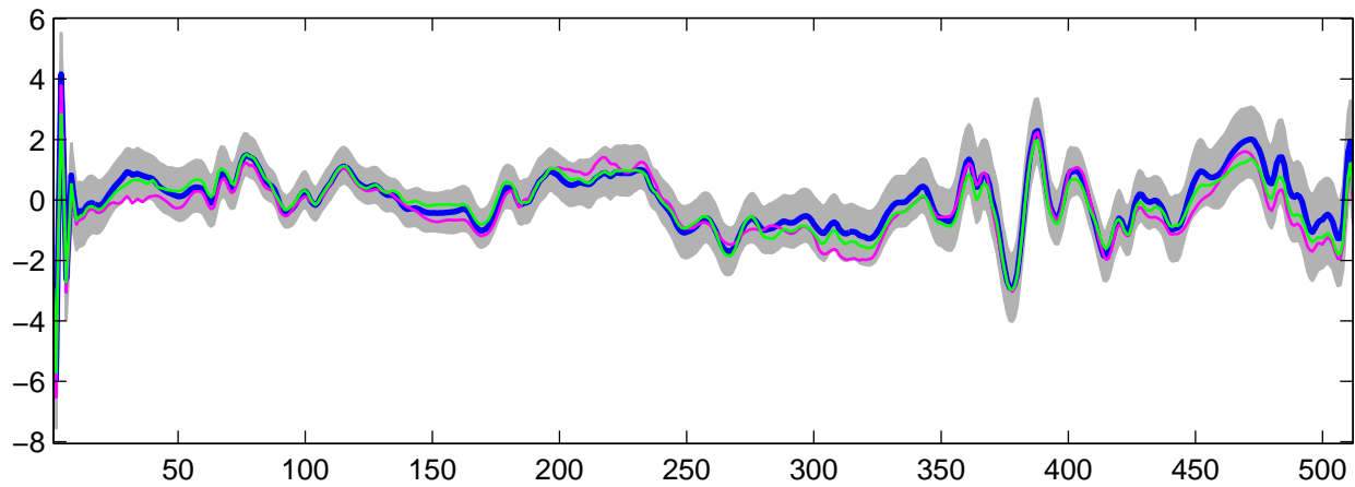
Estimated U_{10}(t) using G-WFMM: t_2 data, run 6
