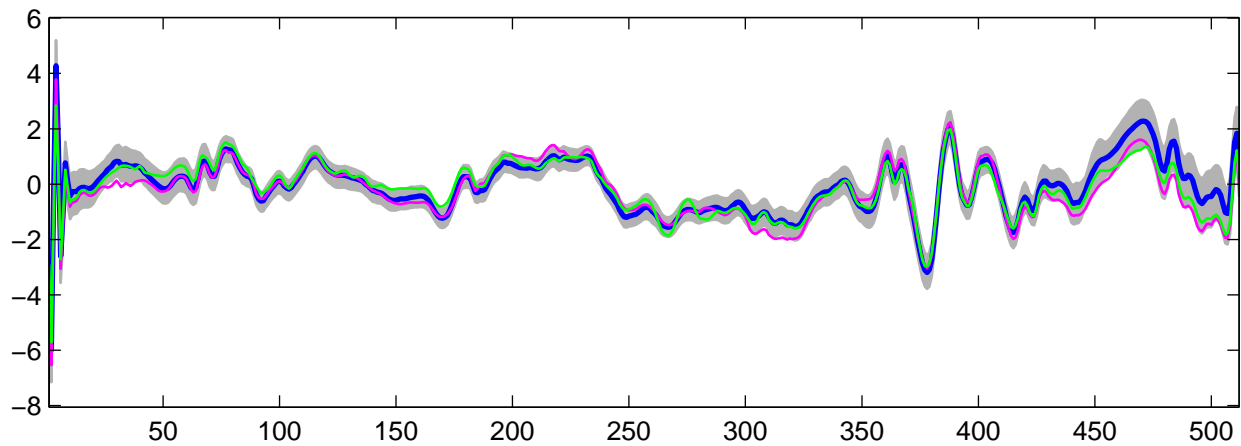
Estimated U_{10}(t) using R-WFMM: t_2 data, run 6
