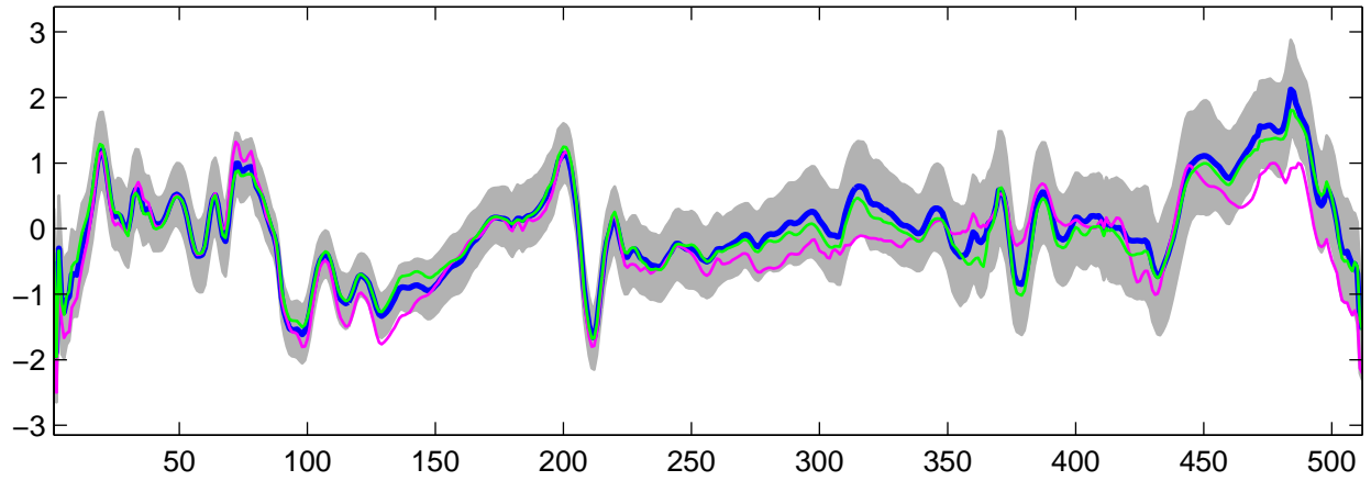
Estimated U_{10}(t) using G-WFMM: t_3 data, run 6
