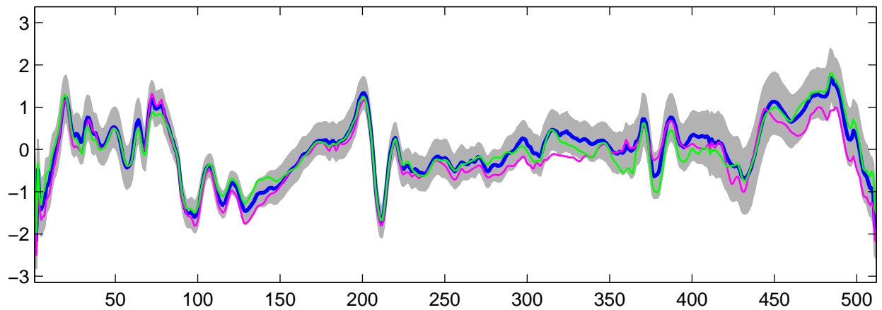
Estimated U_{10}(t) using R-WFMM: t_3 data, run 6
