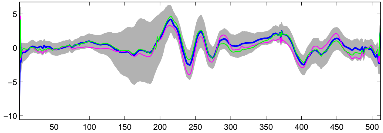
Estimated U_{11}(t) using G-WFMM: t_1 data, run 6
