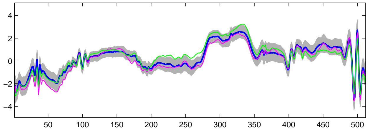
Estimated U_{11}(t) using R-WFMM: t_2 data, run 6
