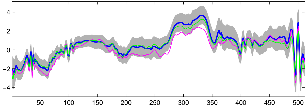
Estimated U_{11}(t) using G-WFMM: t_2 data, run 6
