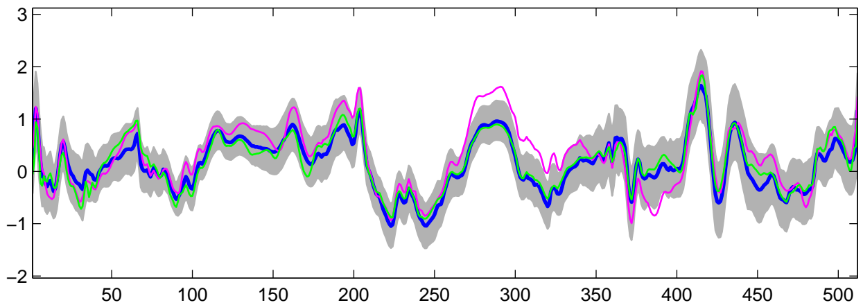
Estimated U_{11}(t) using R-WFMM: t_3 data, run 6
