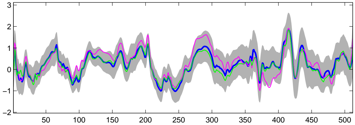
Estimated U_{11}(t) using G-WFMM: t_3 data, run 6
