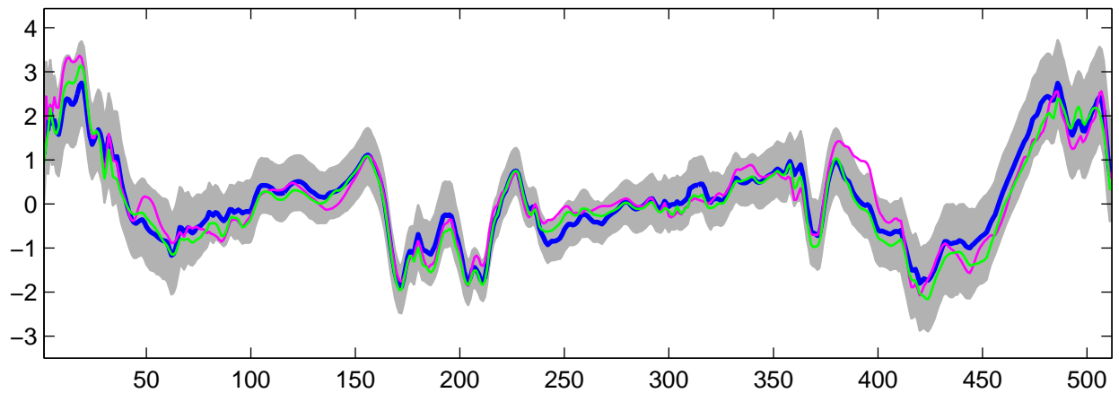
Estimated U_{12}(t) using R-WFMM: Normal data, run 6
