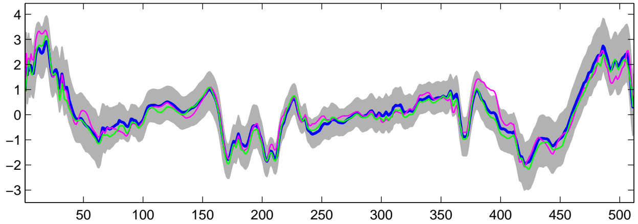
Estimated U_{12}(t) using G-WFMM: Normal data, run 6
