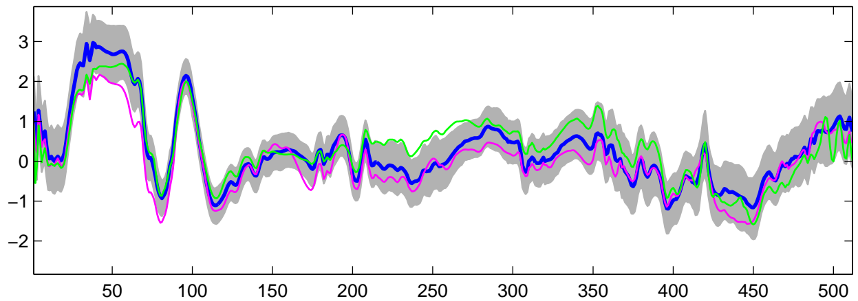
Estimated U_{12}(t) using R-WFMM: t_2 data, run 6
