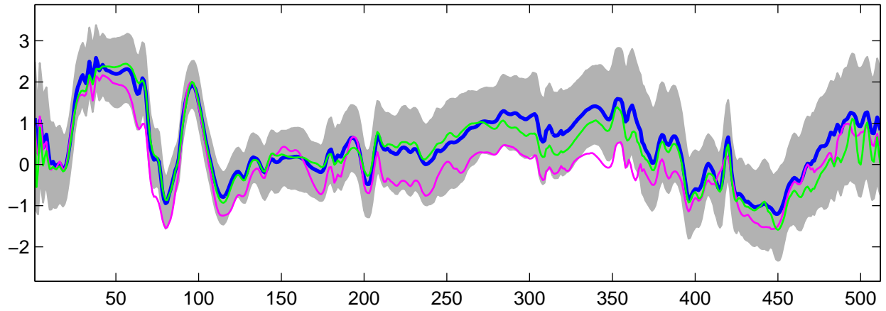
Estimated U_{12}(t) using G-WFMM: t_2 data, run 6
