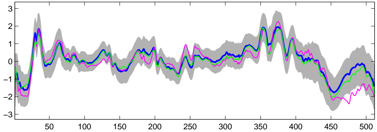
Estimated U_{13}(t) using G-WFMM: DE data, run 6
