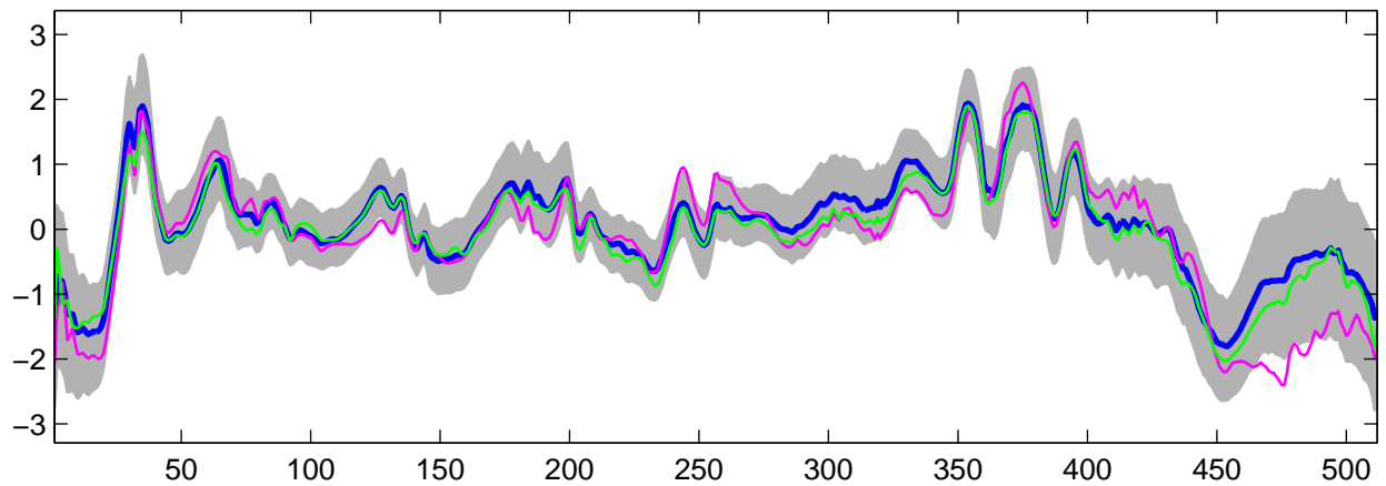
Estimated U_{13}(t) using R-WFMM: DE data, run 6
