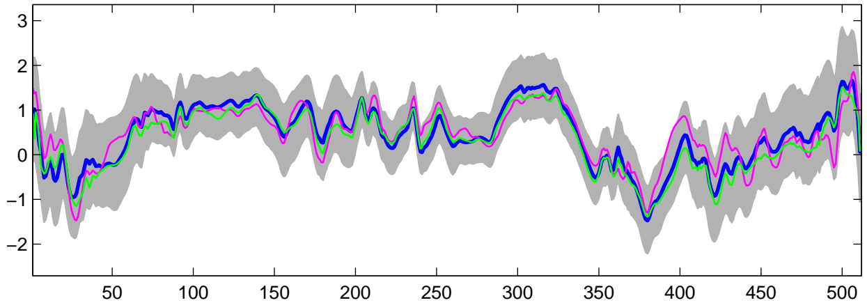
Estimated U_{13}(t) using G-WFMM: Normal data, run 6
