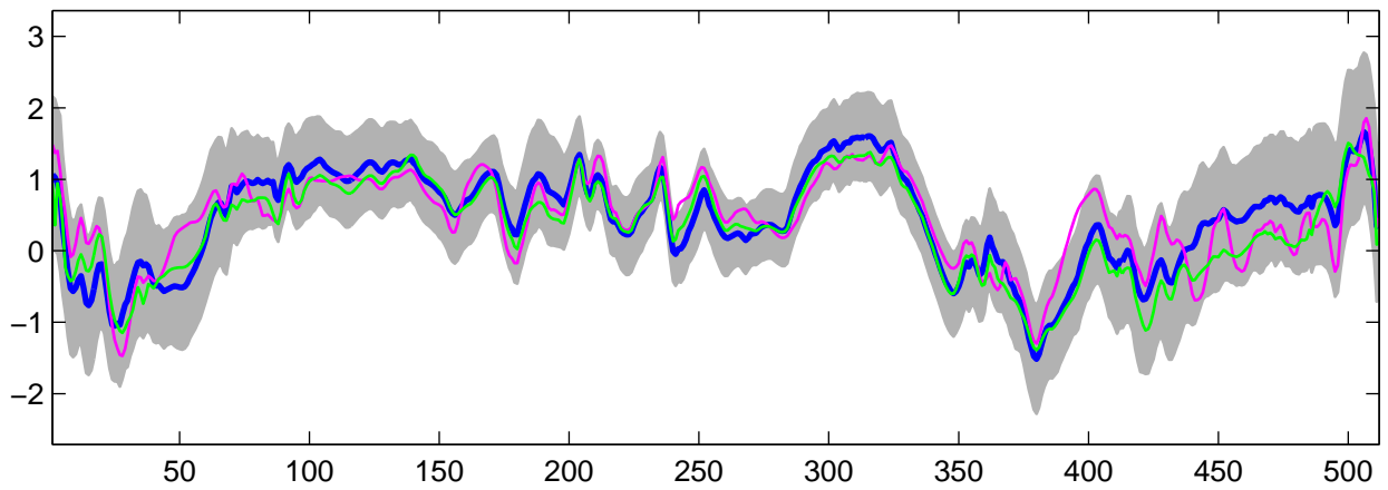
Estimated U_{13}(t) using R-WFMM: Normal data, run 6
