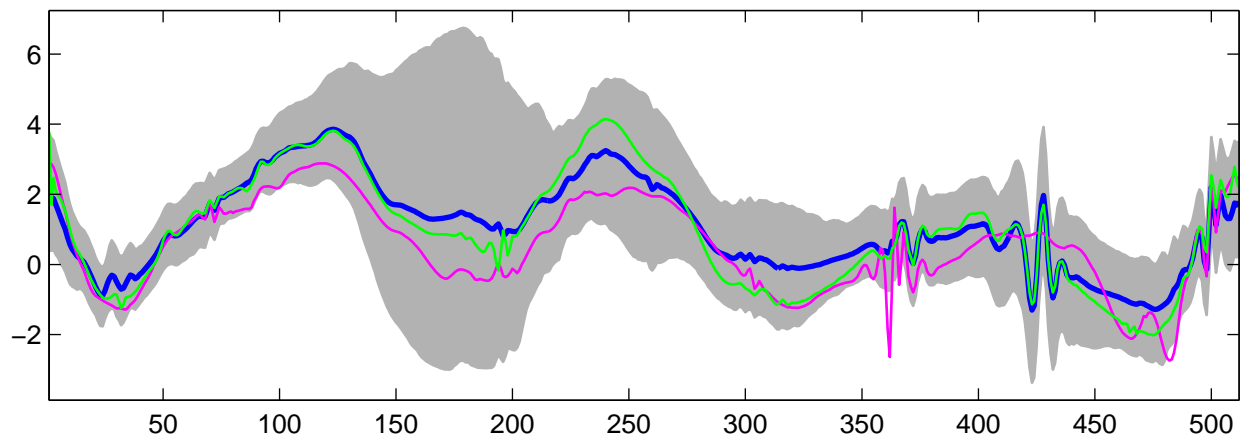
Estimated U_{13}(t) using G-WFMM: t_1 data, run 6
