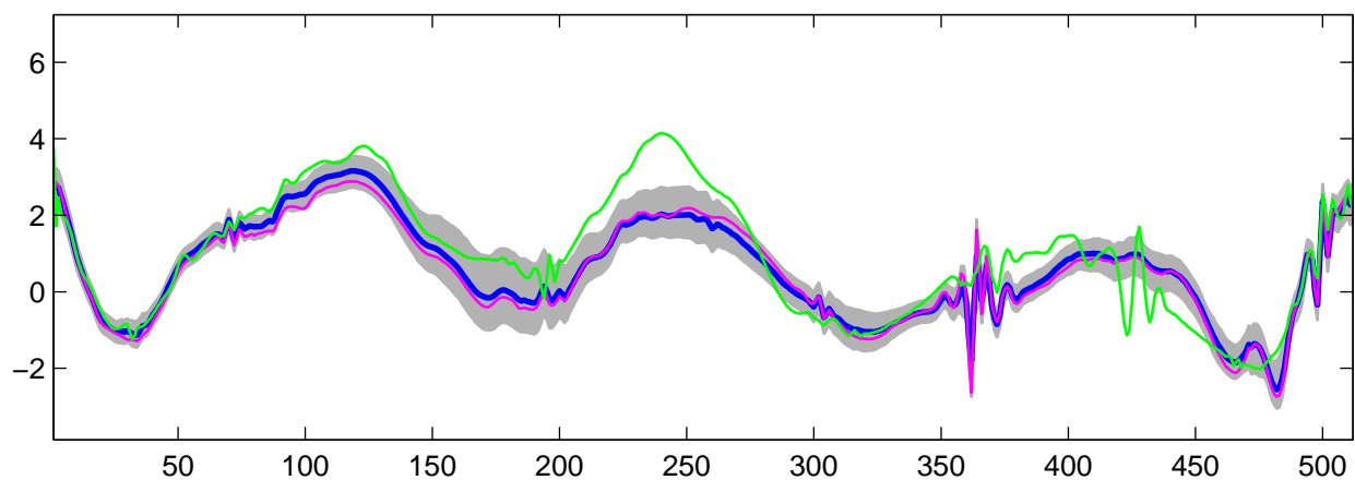
Estimated U_{13}(t) using R-WFMM: t_1 data, run 6
