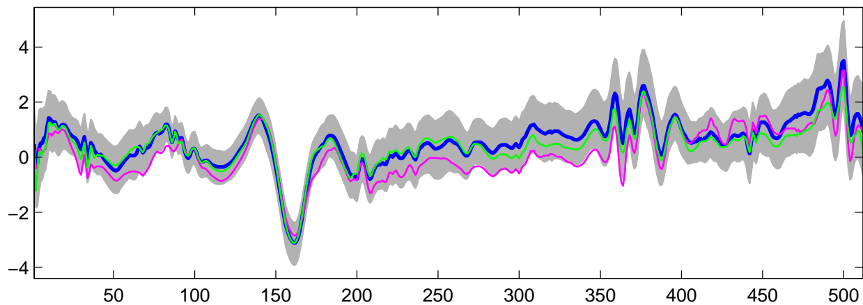
Estimated U_{13}(t) using G-WFMM: t_2 data, run 6
