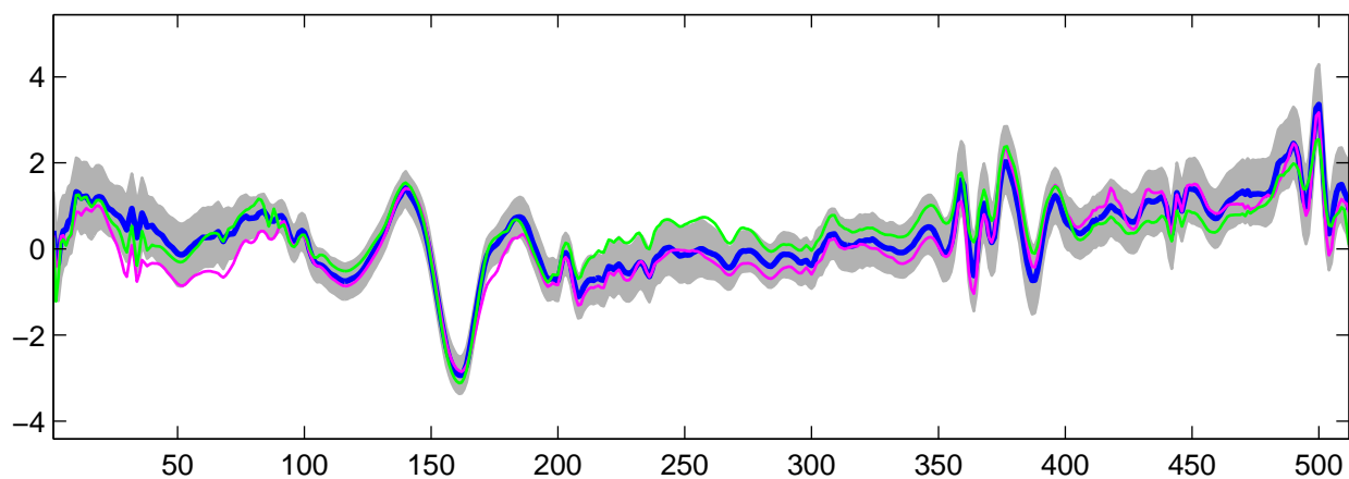
Estimated U_{13}(t) using R-WFMM: t_2 data, run 6
