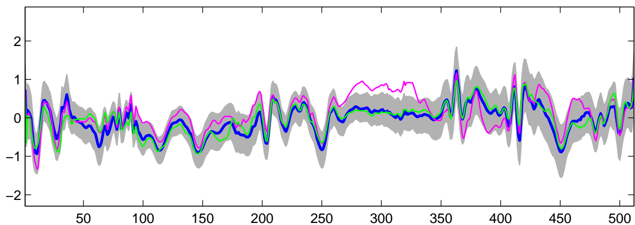
Estimated U_{13}(t) using R-WFMM: t_3 data, run 6
