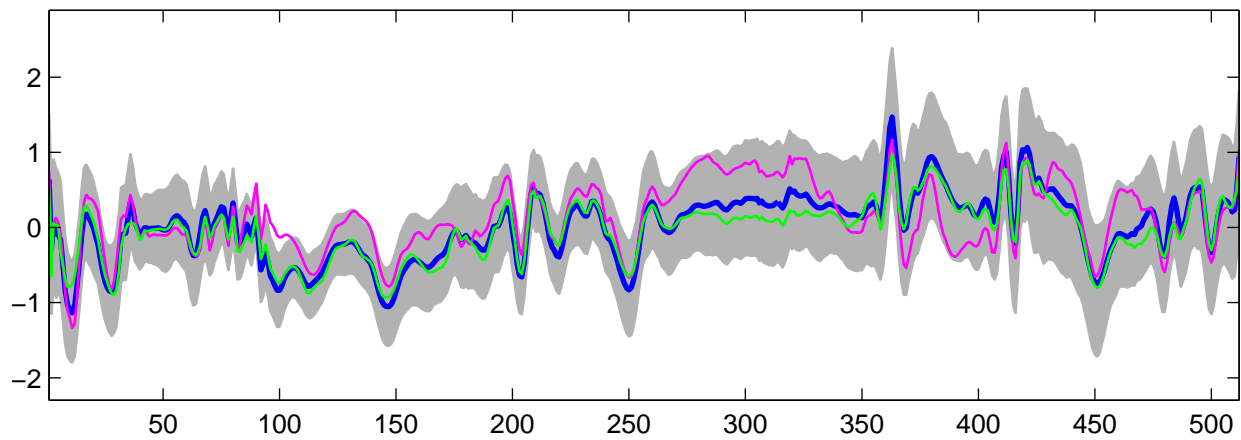
Estimated U_{13}(t) using G-WFMM: t_3 data, run 6
