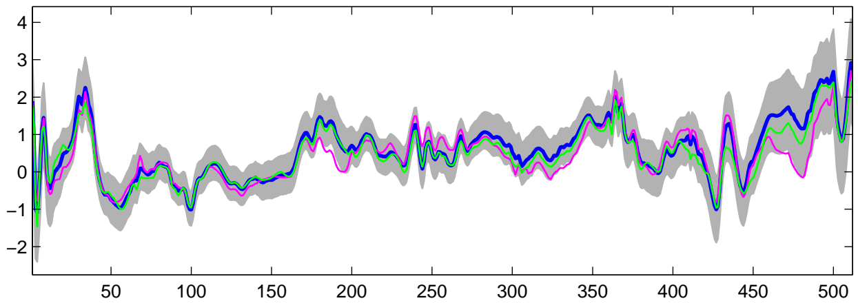
Estimated U_{14}(t) using R-WFMM: DE data, run 6
