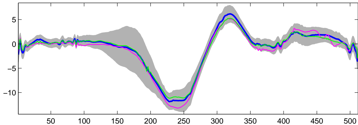
Estimated U_{14}(t) using G-WFMM: t_1 data, run 6
