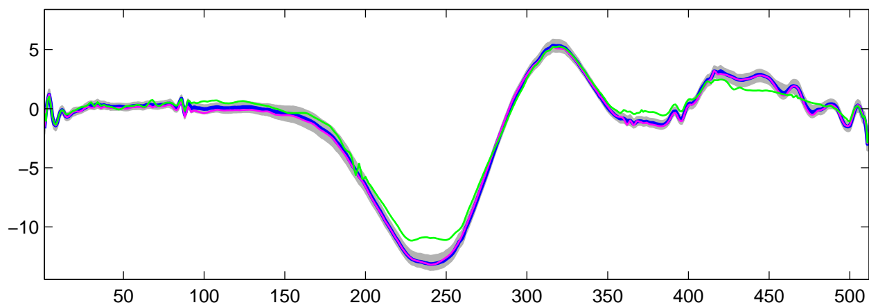
Estimated U_{14}(t) using R-WFMM: t_1 data, run 6
