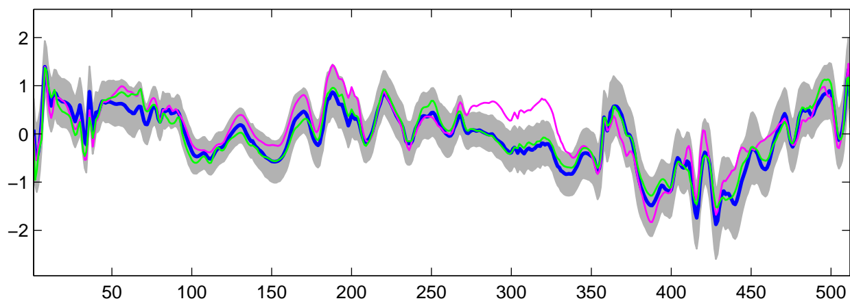
Estimated U_{14}(t) using R-WFMM: t_3 data, run 6
