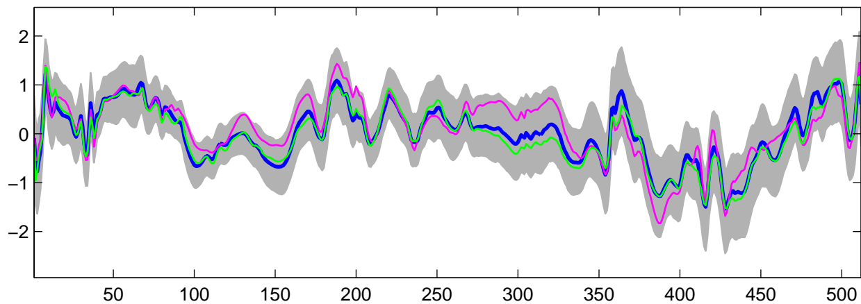
Estimated U_{14}(t) using G-WFMM: t_3 data, run 6
