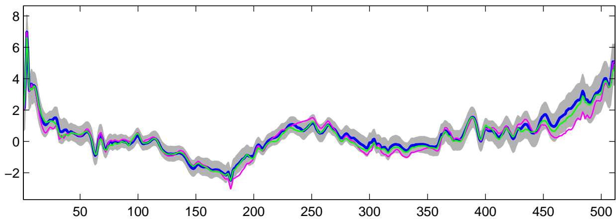
Estimated U_{15}(t) using R-WFMM: DE data, run 6
