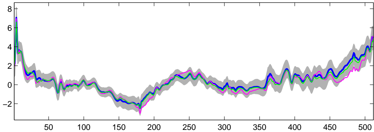
Estimated U_{15}(t) using G-WFMM: DE data, run 6
