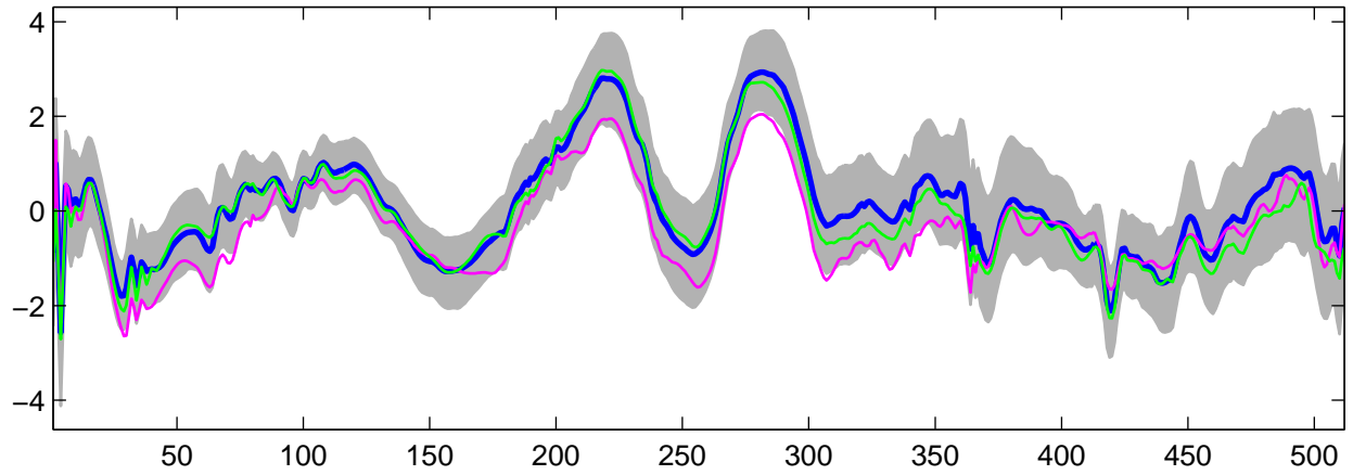
Estimated U_{15}(t) using G-WFMM: t_2 data, run 6
