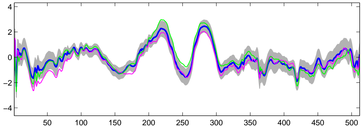
Estimated U_{15}(t) using R-WFMM: t_2 data, run 6
