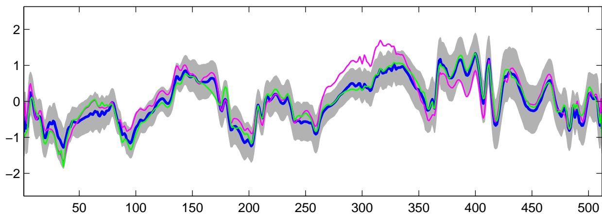
Estimated U_{15}(t) using R-WFMM: t_3 data, run 6
