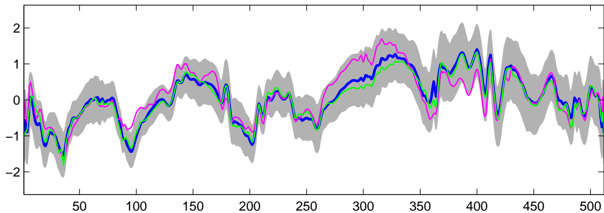
Estimated U_{15}(t) using G-WFMM: t_3 data, run 6
