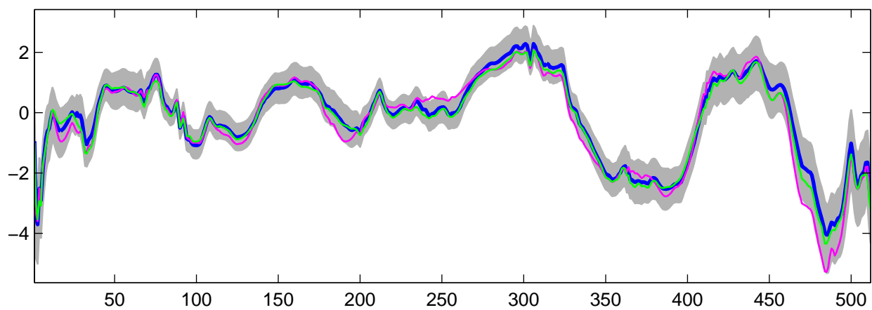
Estimated U_{16}(t) using R-WFMM: DE data, run 6
