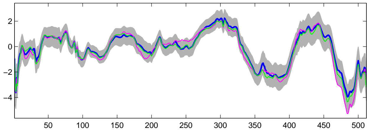
Estimated U_{16}(t) using G-WFMM: DE data, run 6
