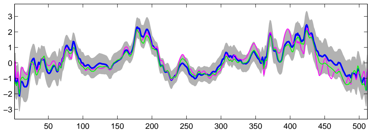
Estimated U_{16}(t) using R-WFMM: Normal data, run 6
