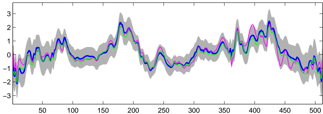
Estimated U_{16}(t) using G-WFMM: Normal data, run 6
