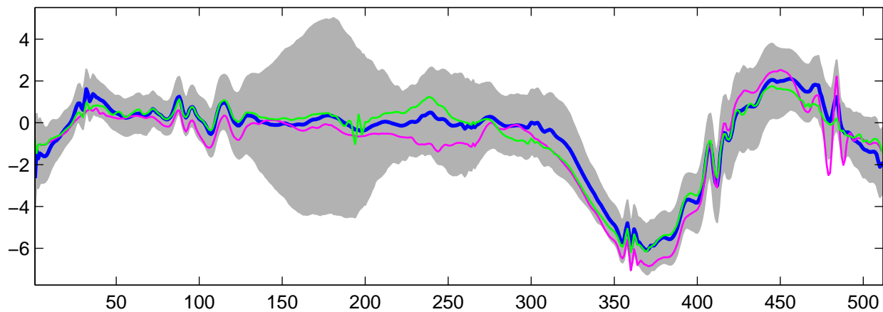
Estimated U_{16}(t) using G-WFMM: t_1 data, run 6
