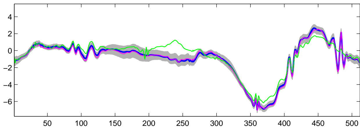
Estimated U_{16}(t) using R-WFMM: t_1 data, run 6
