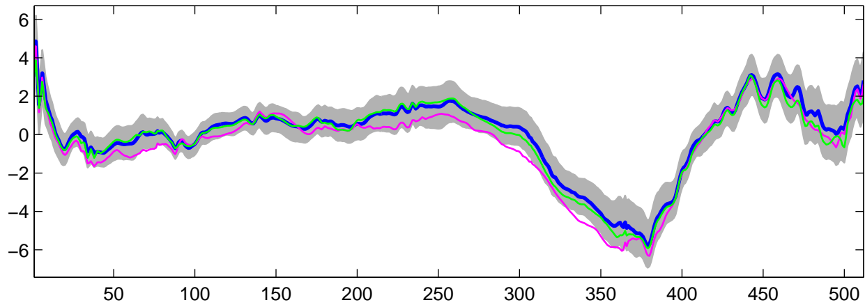
Estimated U_{16}(t) using G-WFMM: t_2 data, run 6
