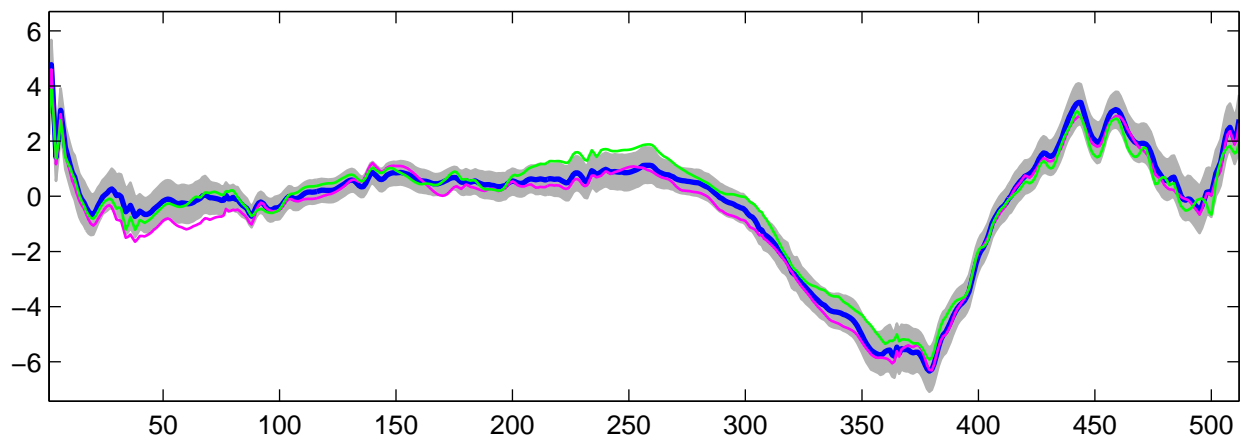
Estimated U_{16}(t) using R-WFMM: t_2 data, run 6
