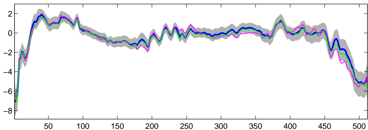
Estimated U_{17}(t) using R-WFMM: DE data, run 6
