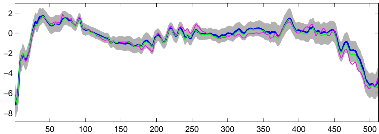
Estimated U_{17}(t) using G-WFMM: DE data, run 6
