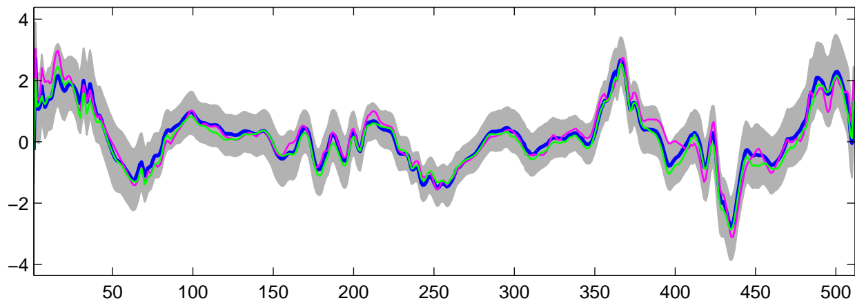
Estimated U_{17}(t) using G-WFMM: Normal data, run 6
