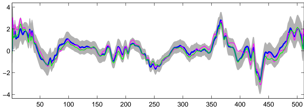
Estimated U_{17}(t) using R-WFMM: Normal data, run 6
