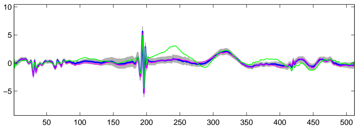
Estimated U_{17}(t) using R-WFMM: t_1 data, run 6
