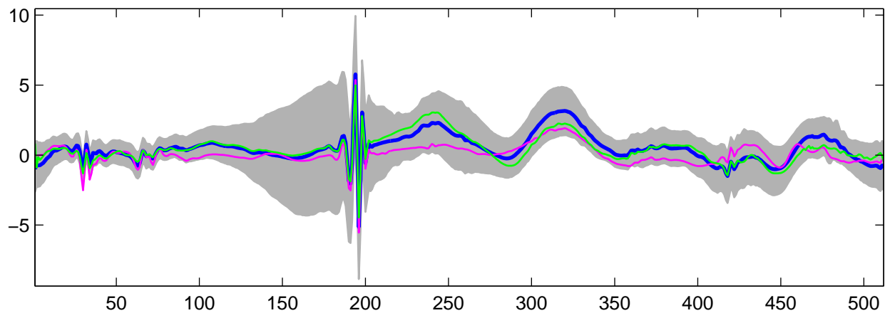
Estimated U_{17}(t) using G-WFMM: t_1 data, run 6
