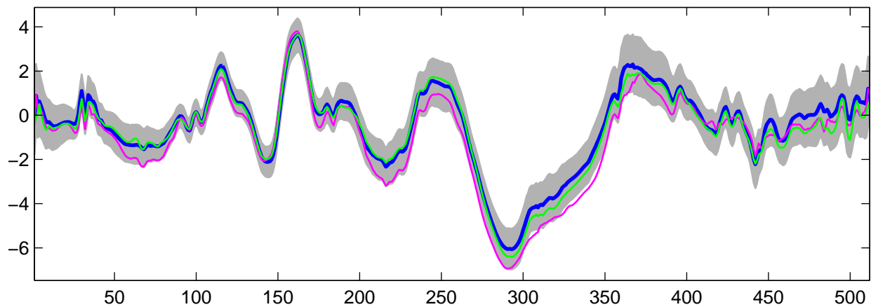
Estimated U_{17}(t) using G-WFMM: t_2 data, run 6
