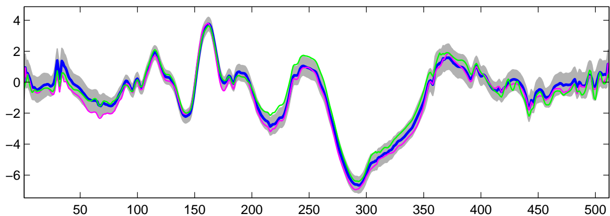
Estimated U_{17}(t) using R-WFMM: t_2 data, run 6
