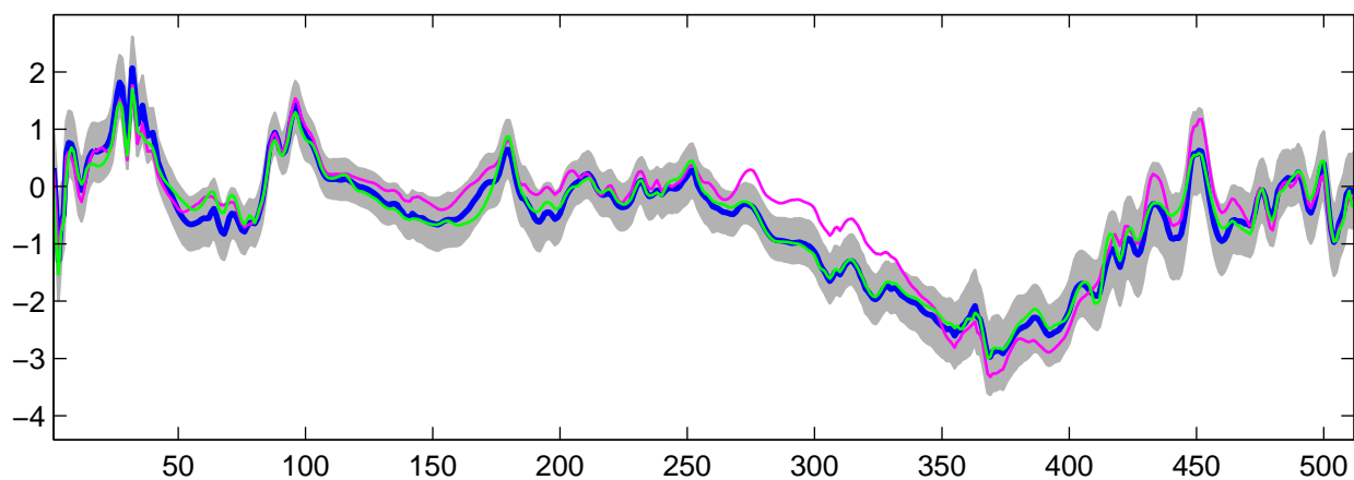
Estimated U_{17}(t) using R-WFMM: t_3 data, run 6
