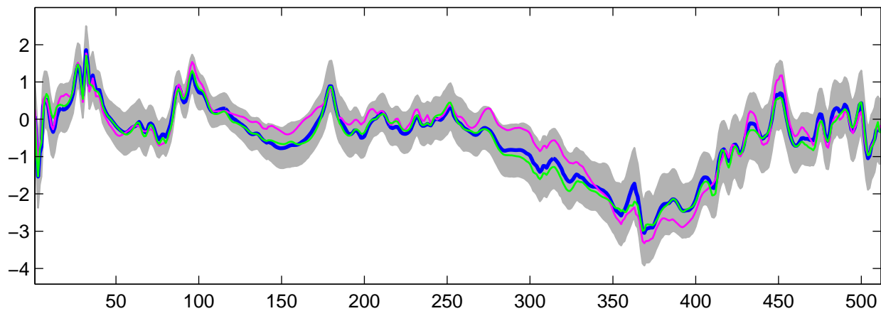
Estimated U_{17}(t) using G-WFMM: t_3 data, run 6
