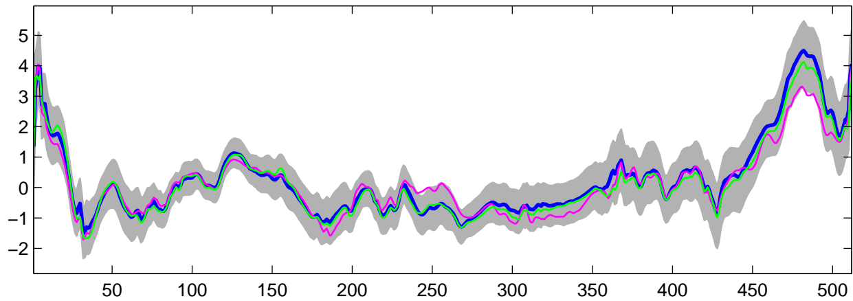
Estimated U_{18}(t) using G-WFMM: DE data, run 6
