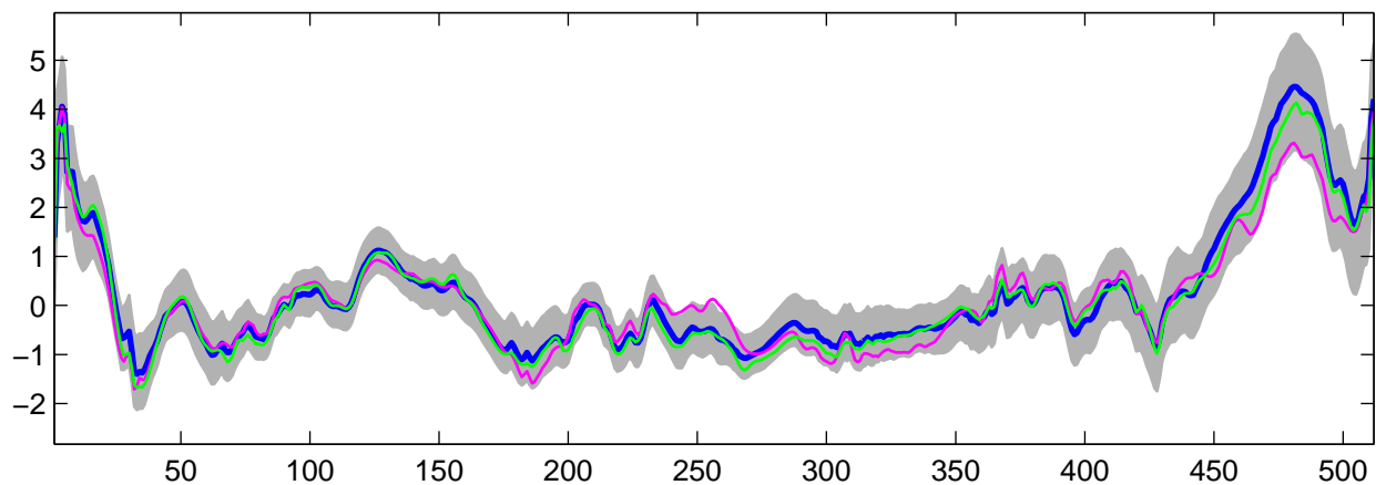
Estimated U_{18}(t) using R-WFMM: DE data, run 6
