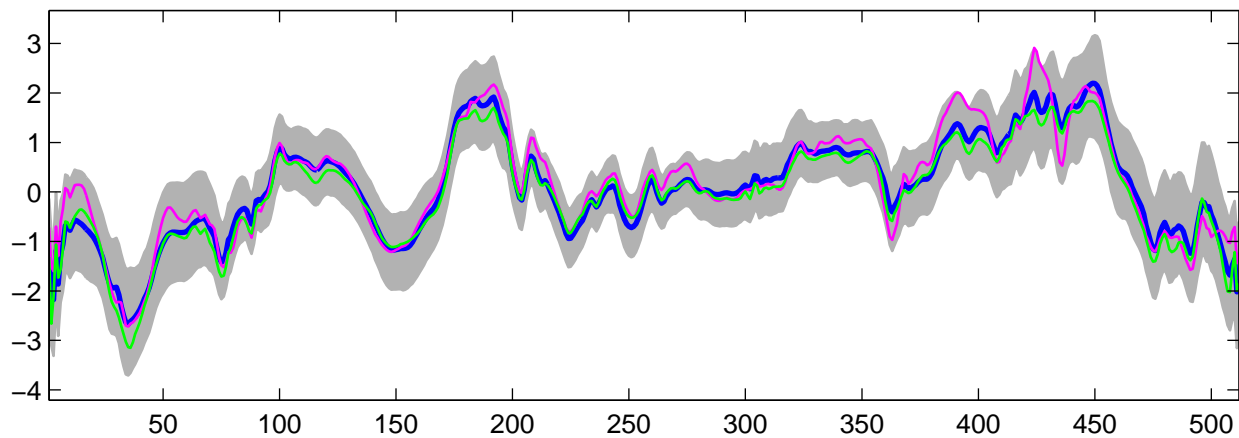
Estimated U_{18}(t) using G-WFMM: Normal data, run 6
