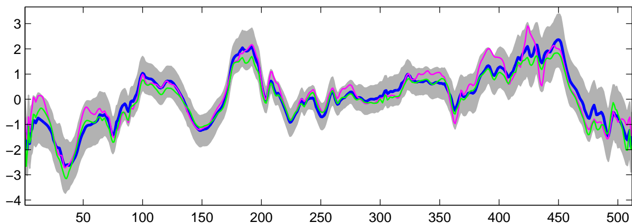
Estimated U_{18}(t) using R-WFMM: Normal data, run 6
