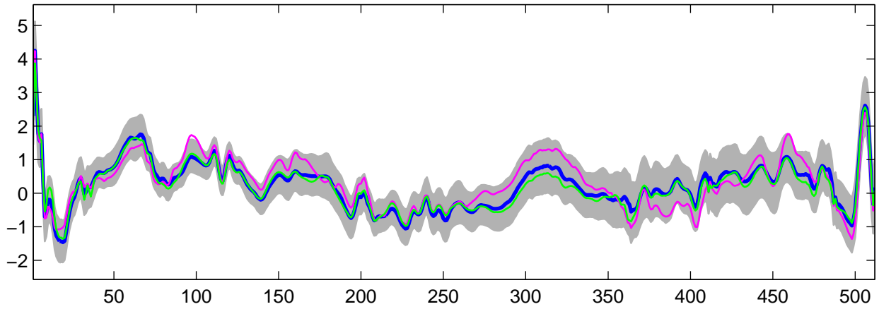
Estimated U_{18}(t) using G-WFMM: t_3 data, run 6
