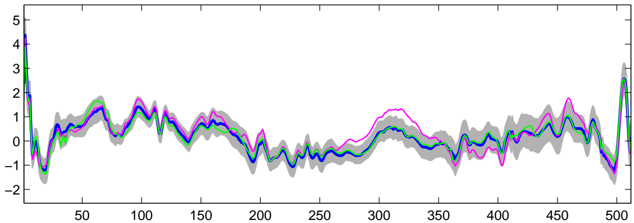
Estimated U_{18}(t) using R-WFMM: t_3 data, run 6
